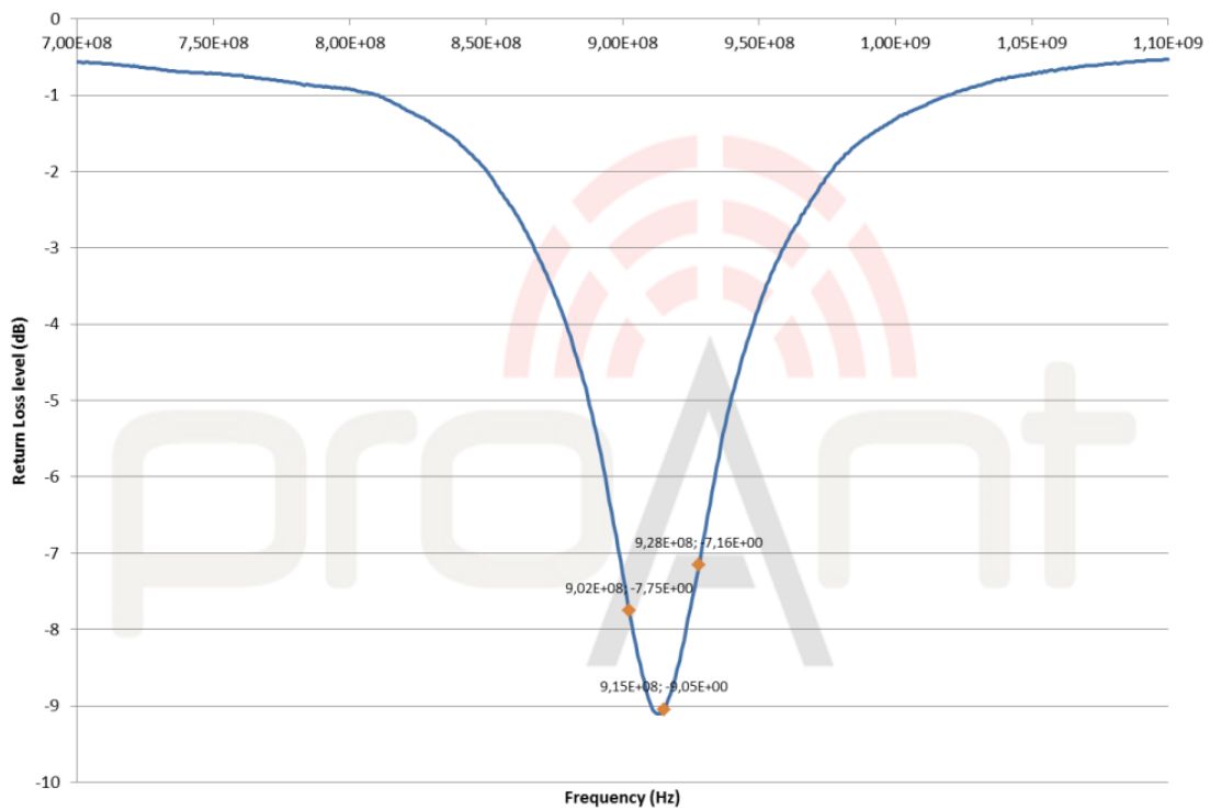
Return Loss
