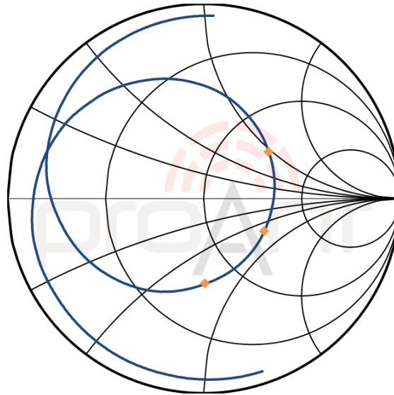
Smith chart
