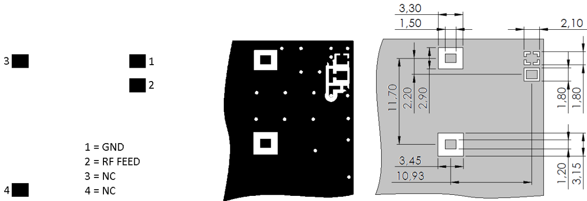
Pin configuration
