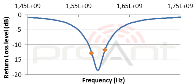
Return Loss
