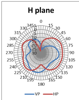
Radiation pattern, 868 MHz
